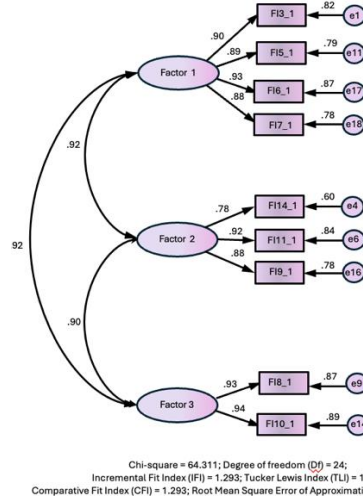
Figure 5. CFA measurement model for digital financial inclusion
