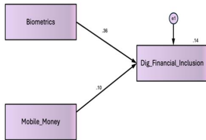
Figure 6. Unmoderated structural equation model in AMOS
